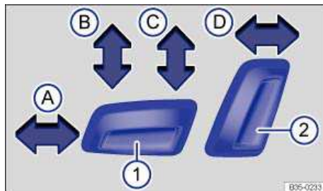
Fig. 46 Driver seat: Controls to adjust the seat backward and forward, adjust seat cushion height and angle, and backrest angle.
