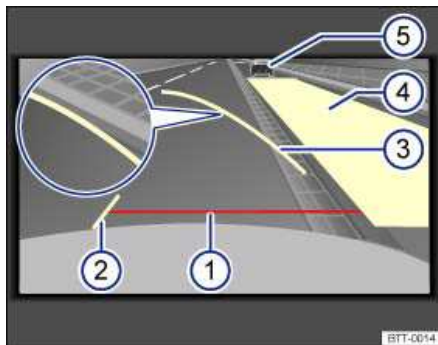
Fig. 155 On screen: Orientation lines and area of the parking space behind the vehicle.
