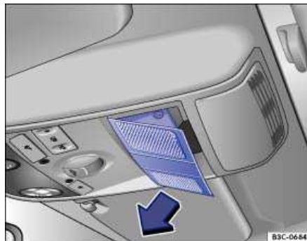
Fig. 180 In headliner: Removing cover.
