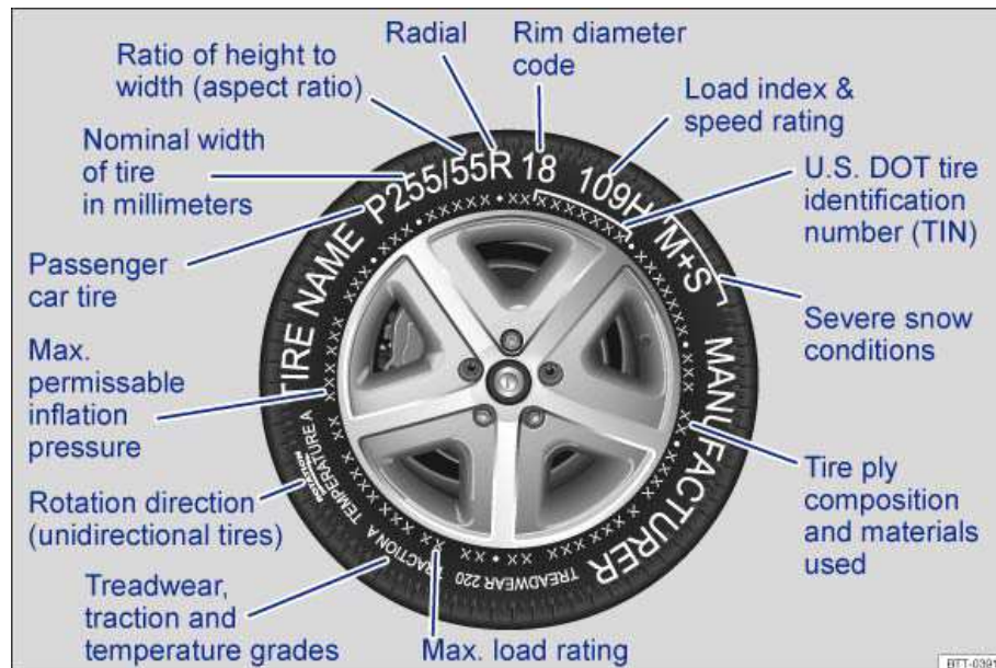
Fig. 116 International tire labeling.
