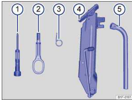
Fig. 185 Contents of the vehicle tool kit.
