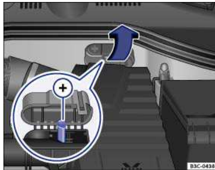
Fig. 210 In the engine compartment: Positive jump start terminal +.
