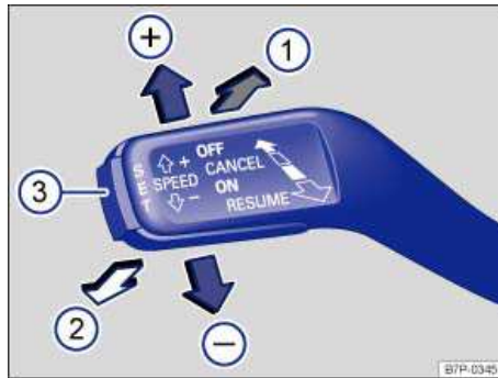
Fig. 151 On the left side of the steering column: Cruise control operating lever.
