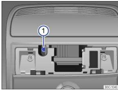
Fig. 181 Hexagonal head screw for closing the power sunroof.
