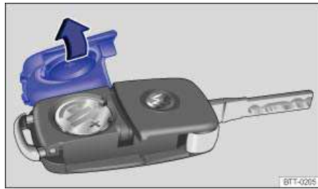
Fig. 23 Remote control vehicle key: Open battery compartment cover.
