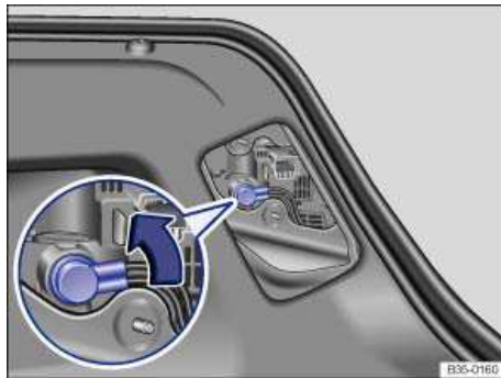
Fig. 207 In the luggage compartment lid: Removing the bulb holder.
