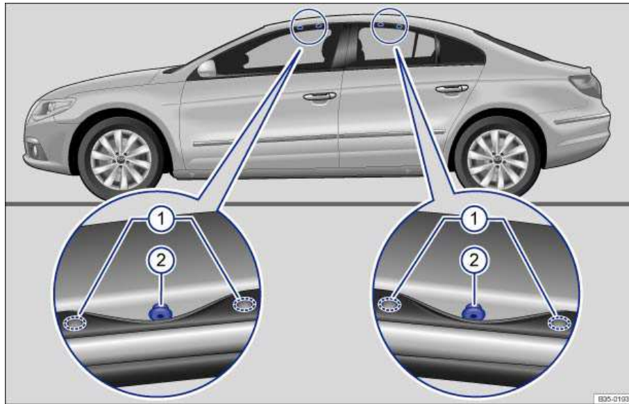
Fig. 107 Under the rubber seal above the front and rear doors: Attachment points for the base carrier.
