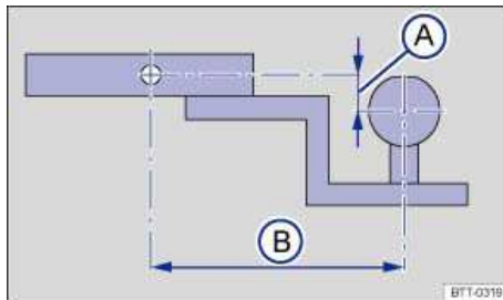
Fig. 108 Dimensions of the ball mount support.
