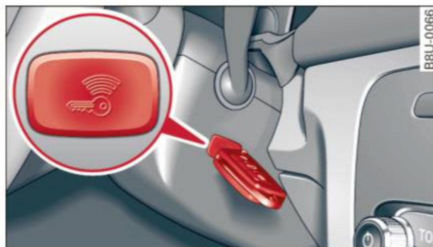
Fig. 71 Steering column/remote control key: starting the engine if there is a malfunction
