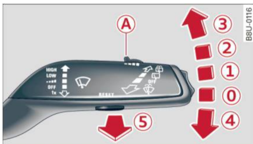
Fig. 41 Windshield wiper lever
