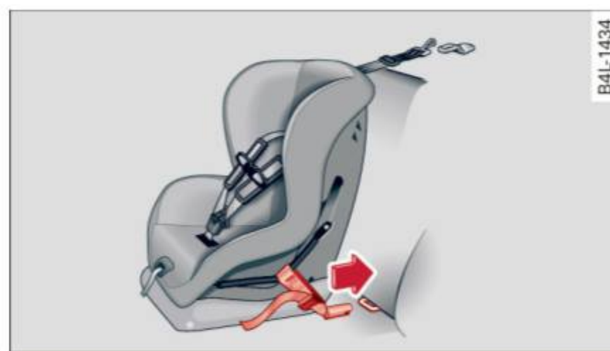
Fig. 131 Lower anchorages: proper mounting
