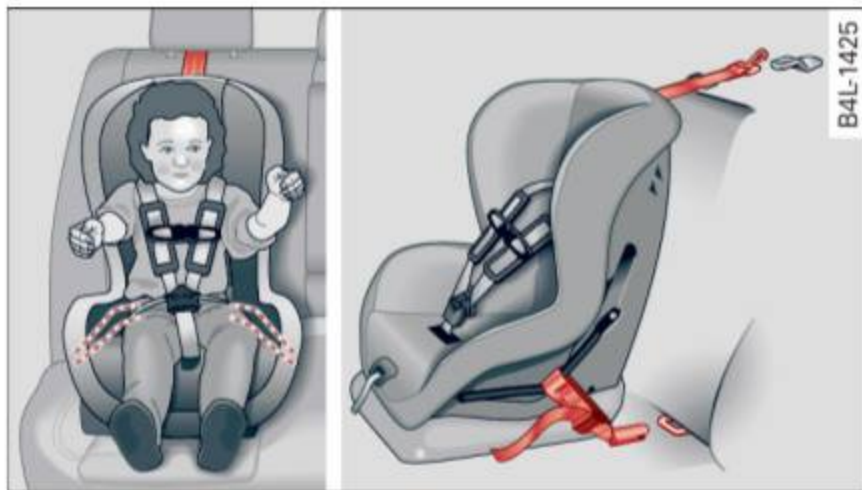
Fig. 125 Schematic overview: installation of the attachments applicable to a LATCH seat
