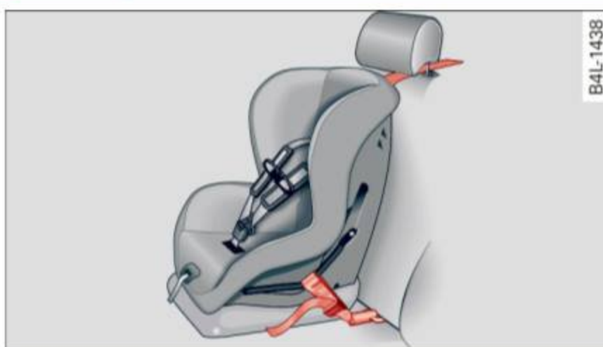
Fig. 133 Tether strap: proper routing and mounting
