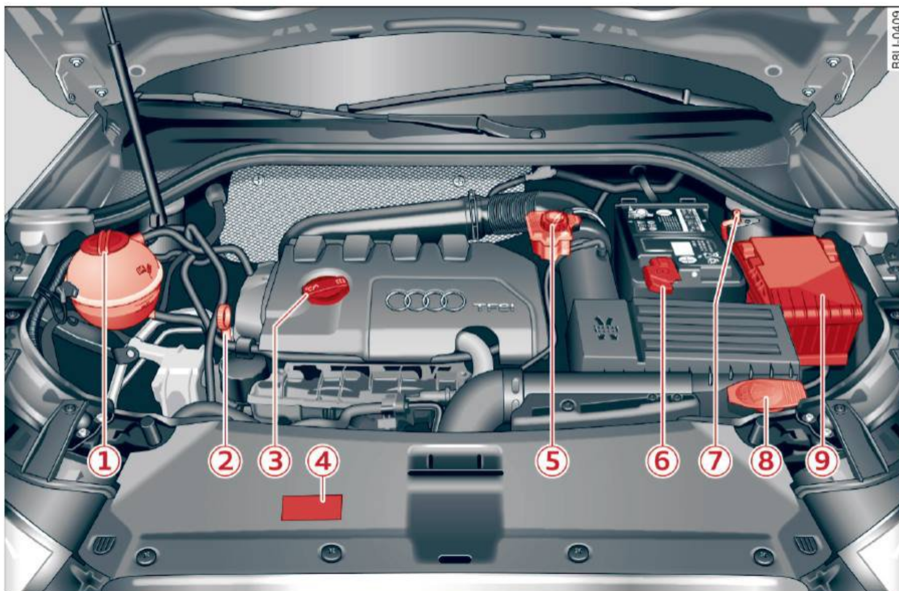
Fig. 140 Typical location of the reservoir and the engine oil filler opening
