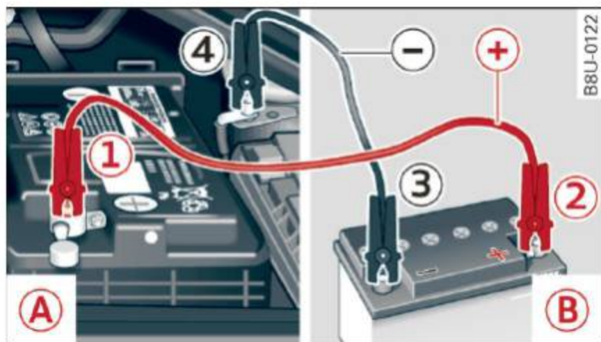
Fig. 165 Jump starting with the battery of another vehicle: (A) discharged vehicle battery, (B) booster battery
