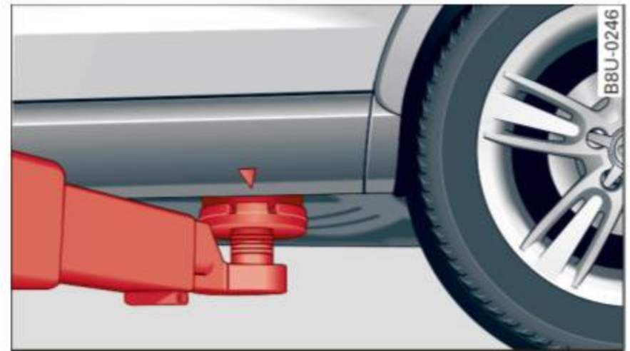
Fig. 172 Rear lifting point
