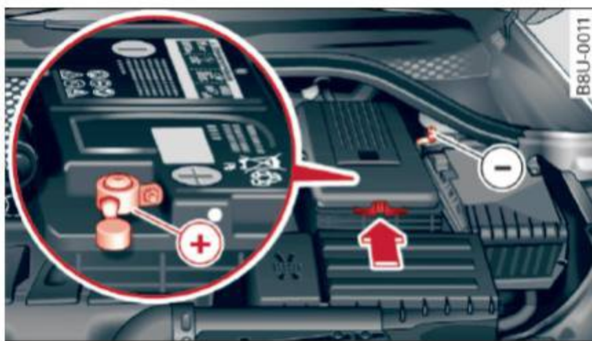
Fig. 145 Engine compartment: connections for a charger and jump start cables
