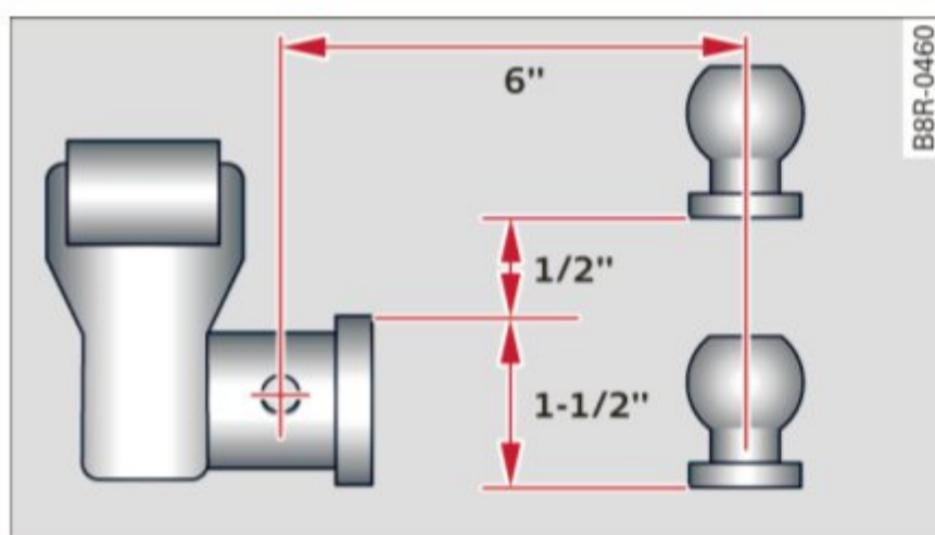
Fig. 79 Permitted ball position of the trailer hitch
