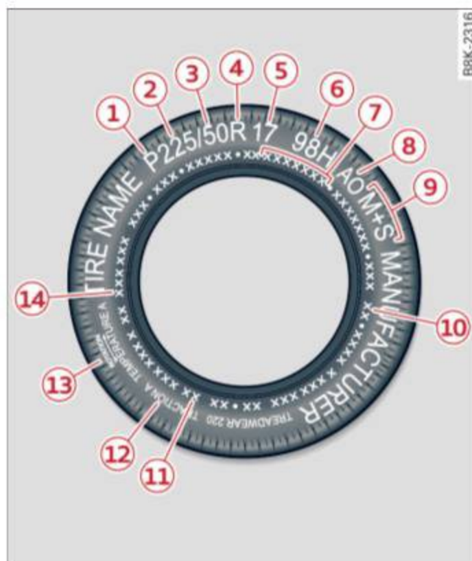
Fig. 147 Tire designations on the side-wall
