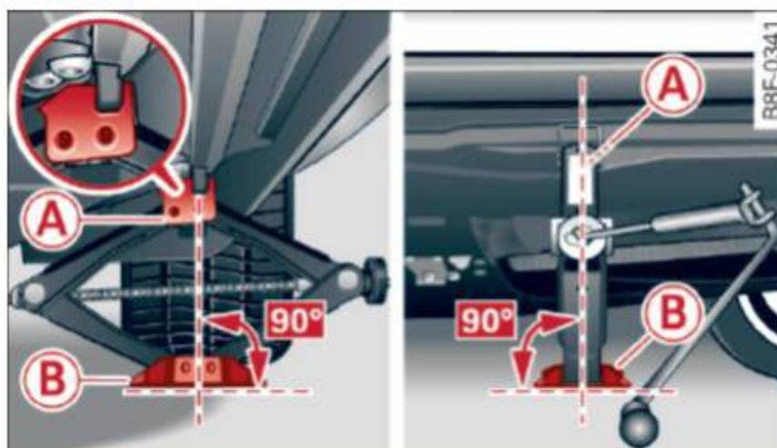
Fig. 157 Sill: positioning the vehicle jack
