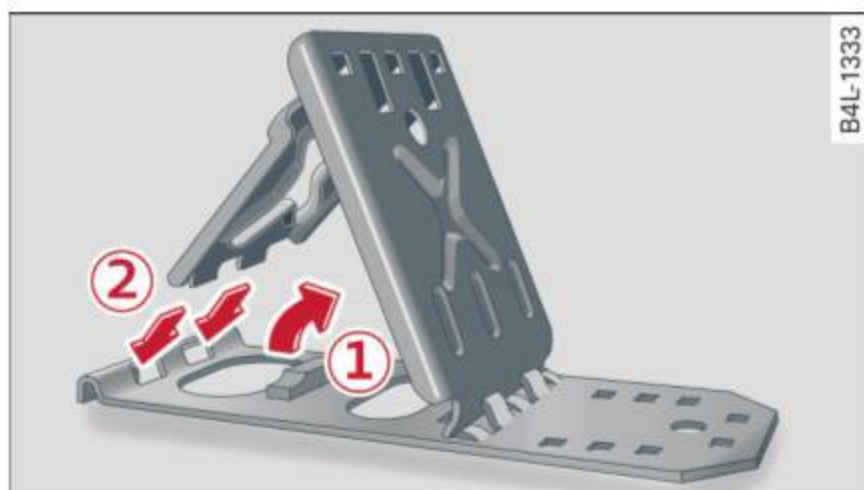
Fig. 152 Opening the folding chocks
