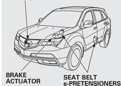
RADAR SENSOR
